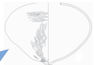
0 (1:20) 50cm
